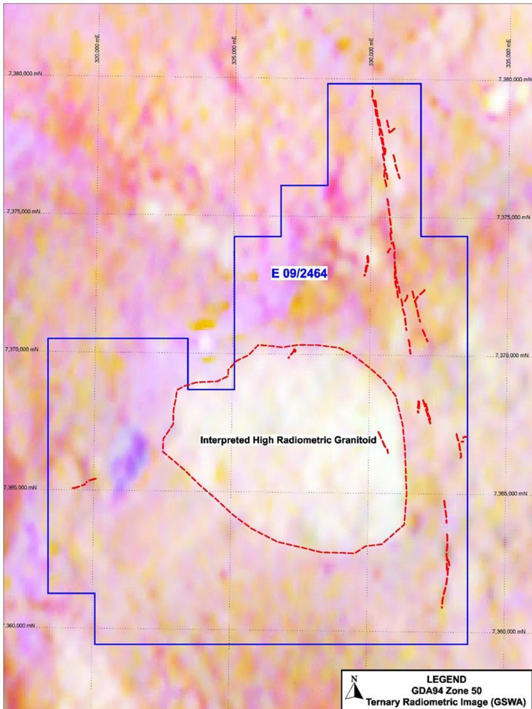
Figure 3: Ternary Radiometric Imagery Willi Creek Project
