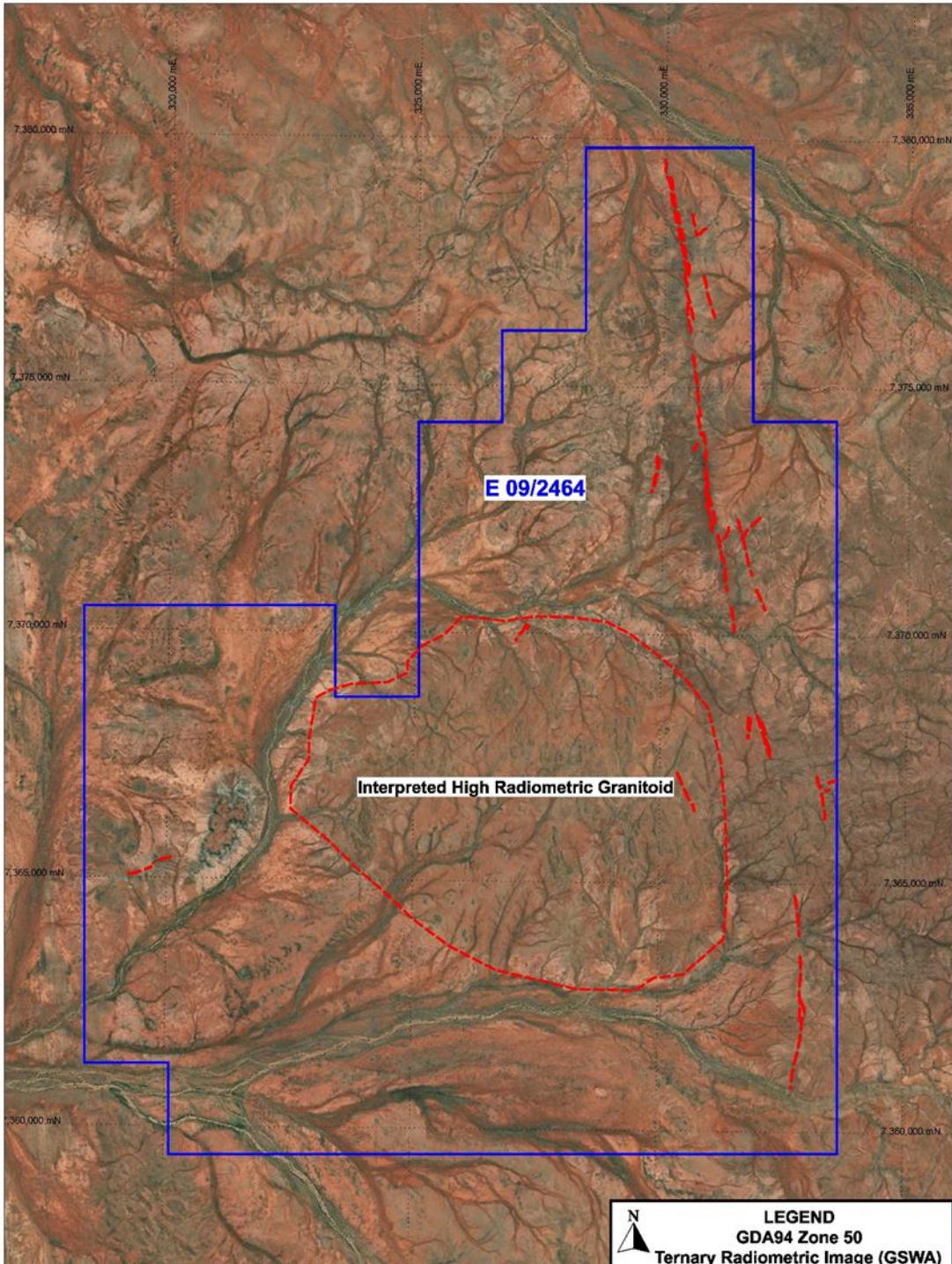
Figure 4: Ternary Imagery and Interpreted Structural Trends: Willi Creek Project
